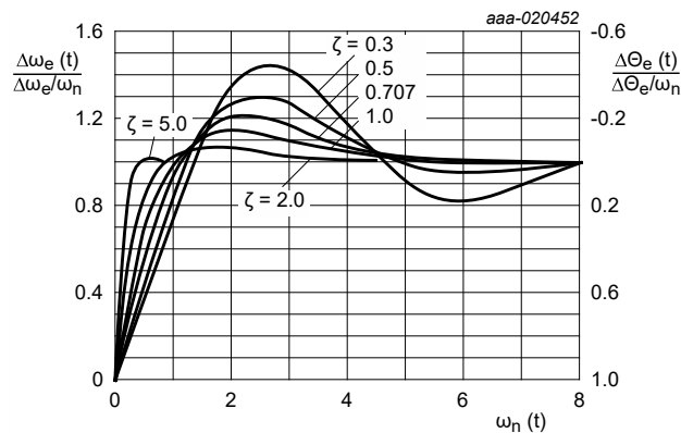
Fig. 35. Type 2, second order frequency step response
